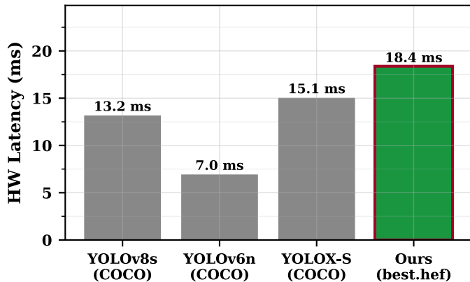
(b) Single-Inference NPU Latency Hailo-8L NPU
