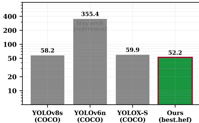
(a) Inference Throughput Hailo-8L NPU
